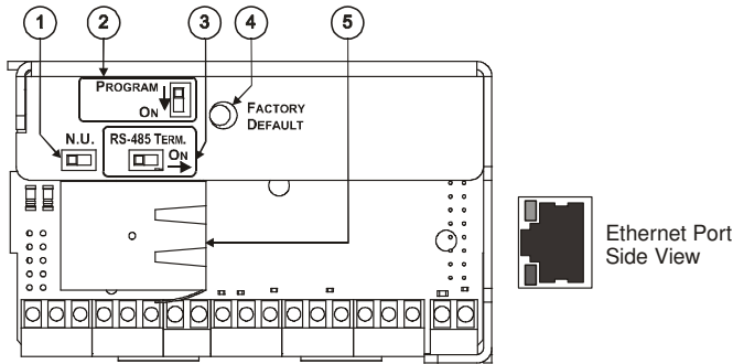
Figure 3: RC-8IRP Rear Panel
