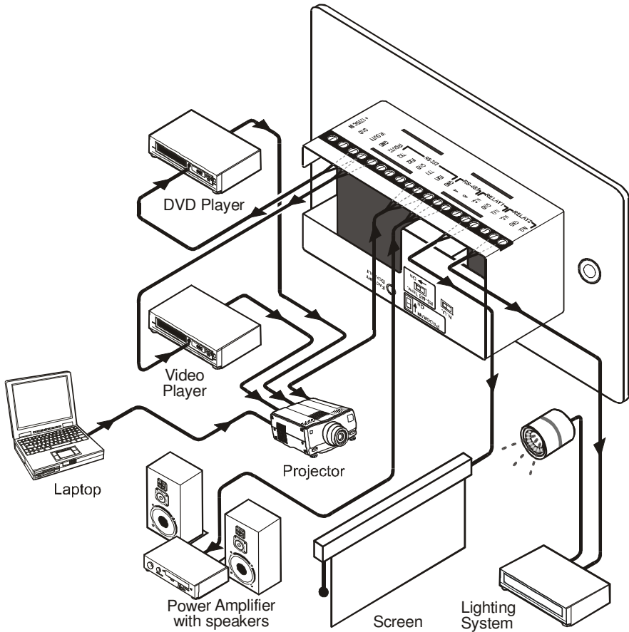
Figure 4: Example of a Typical RC-8IRP Configuration
