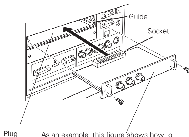
As an example, this figure shows how to install a Dual-SDI Board.
