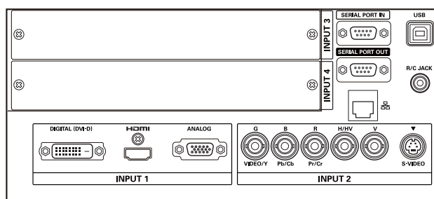
DIGITAL(DVI-D)/HDMI/ANALOG 5-BNC / S-Video jacks Terminals
