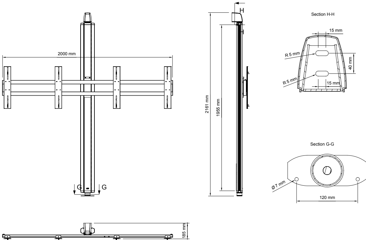
Electrical power sockets can be mounted at the rear.
